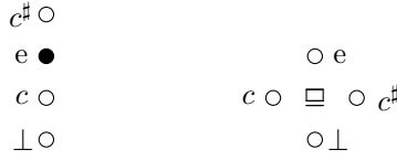
FIGURE 2. The algebra \mathbf{C}_4 .
