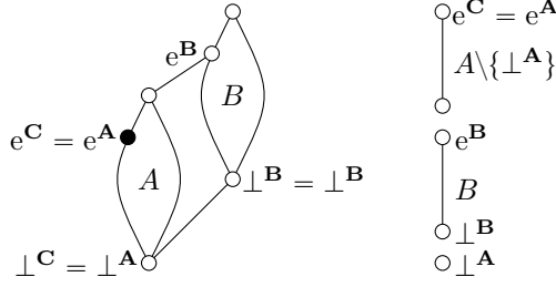
FIGURE 1. The Catalan sum \mathbf{C} = \mathbf{A} \textcircled{C} \mathbf{B} , for nontrivial \mathbf{A} .
